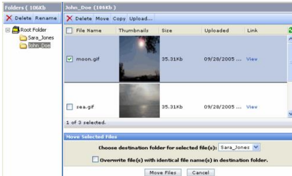
Figure 153 Moving files
