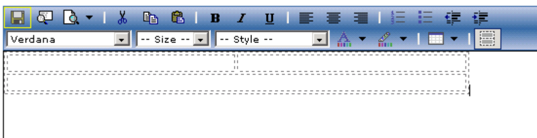
Figure 639 Merged cells
