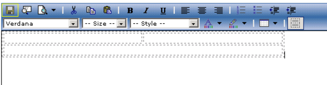
Figure 653 Merged cells
