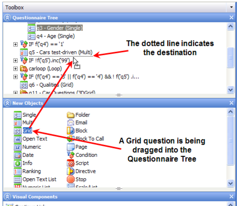
Figure 28 Drag-and-Drop operations
