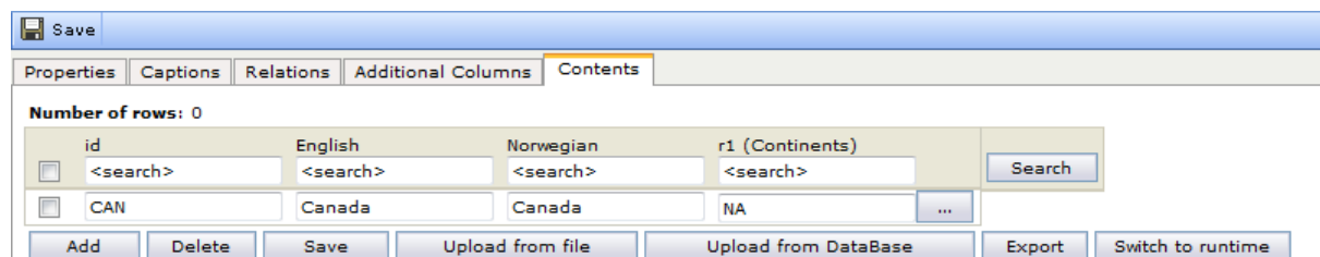
Figure 417 Table contents
