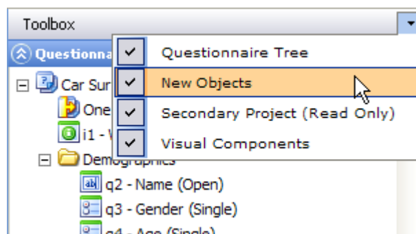
Figure 22 Removing toolboxes
