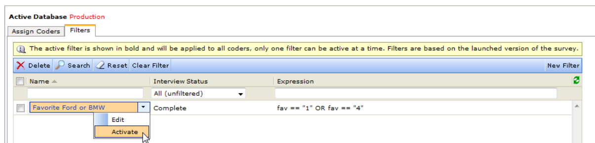
Figure 672 The new filter in the Filters tab list
