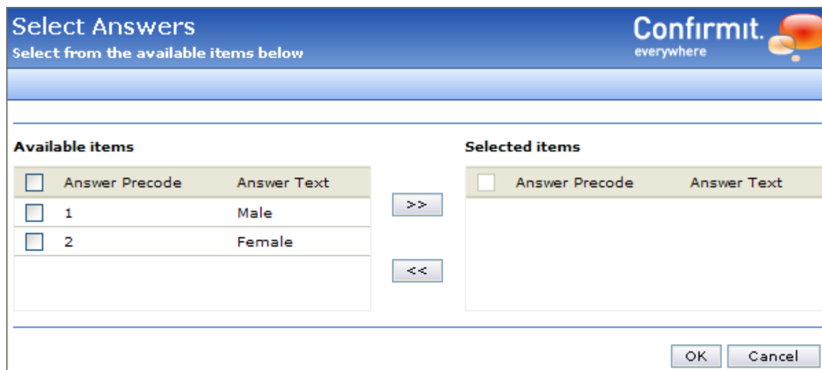
Figure 592 Excluding samples
