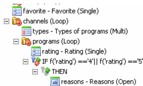
Figure 472 Nested loops
