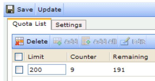
Figure 360 Global Quota
