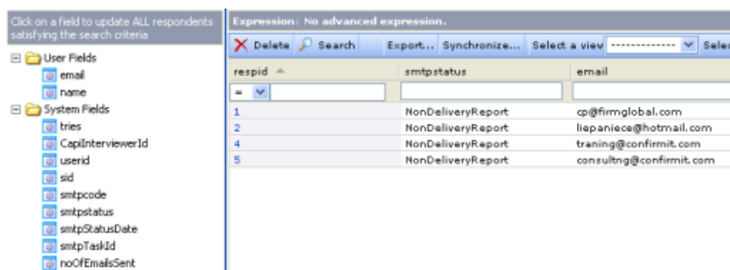
Figure 574 Respondent Editor
