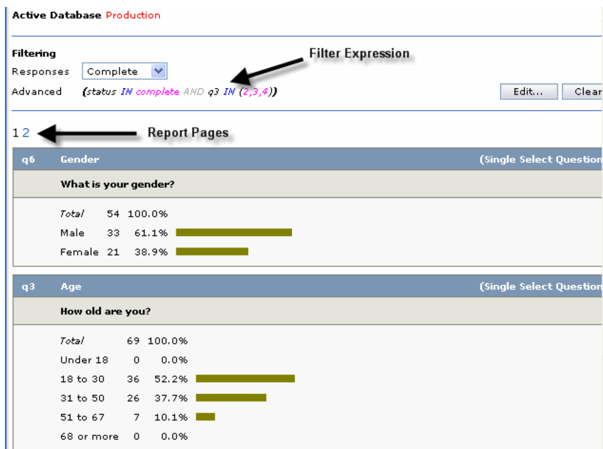
Figure 509 Example of a filtered topline report
