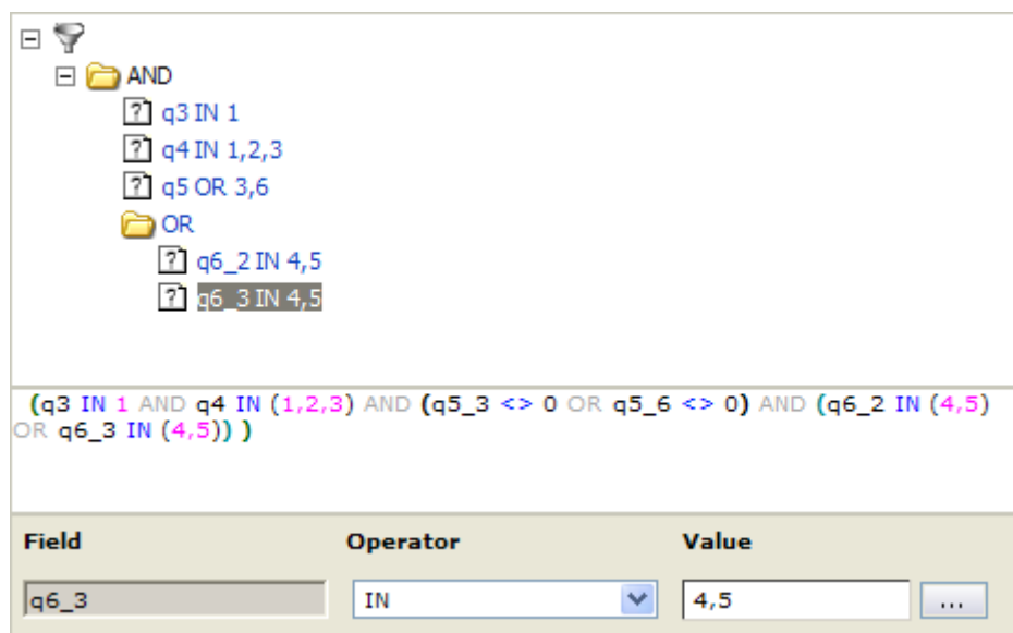
Figure 761 The final filter expression
