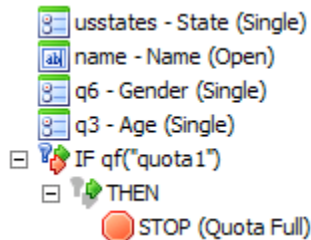
Figure 367 Quota Condition
