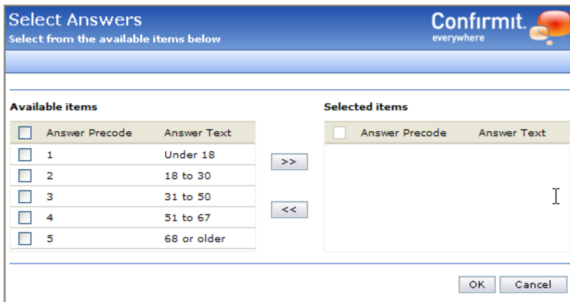
Figure 756 The Select Answers window for the Age element
