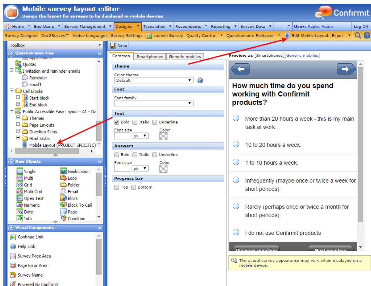
Figure 516 The Mobile Survey Layout Editor page
