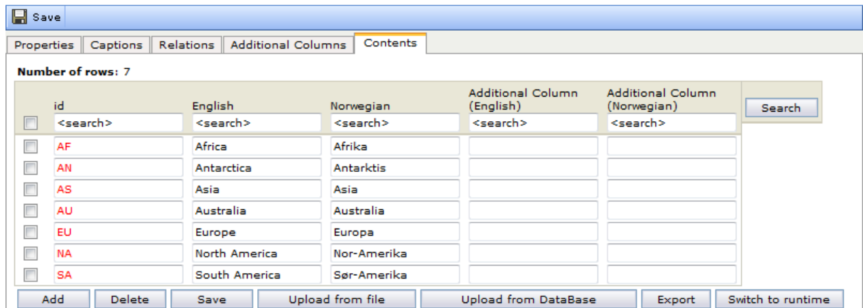
Figure 417 A column is added for each language selected for the table
