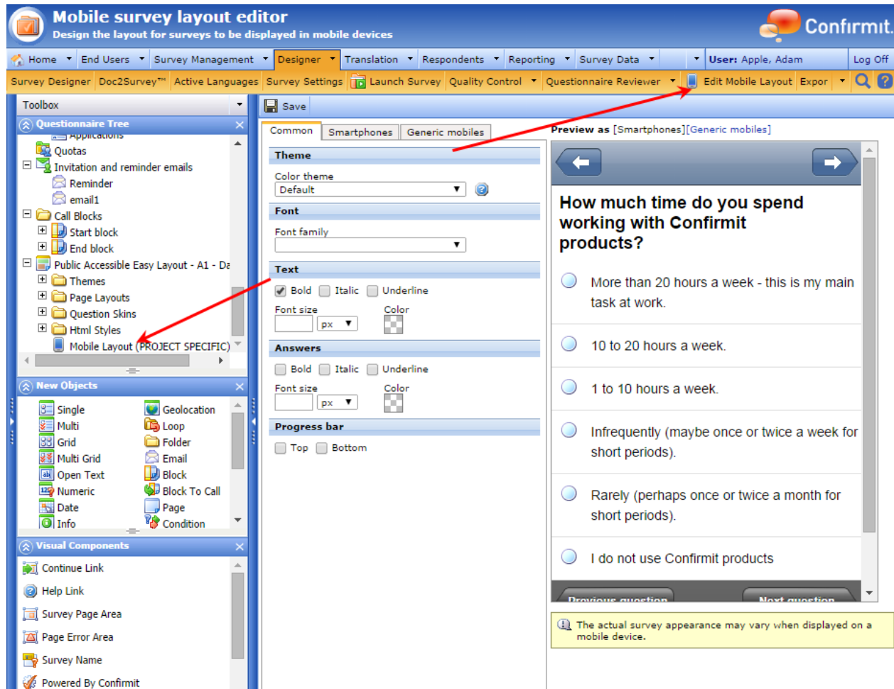
Figure 535 The Mobile Survey Layout Editor page
