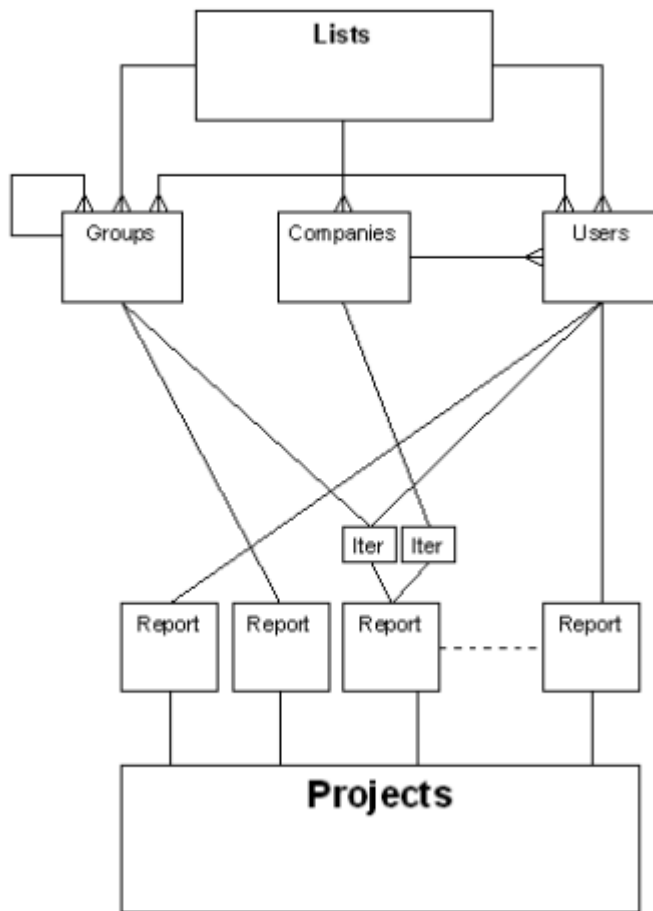
Figure 805 The End User administration interface layout
