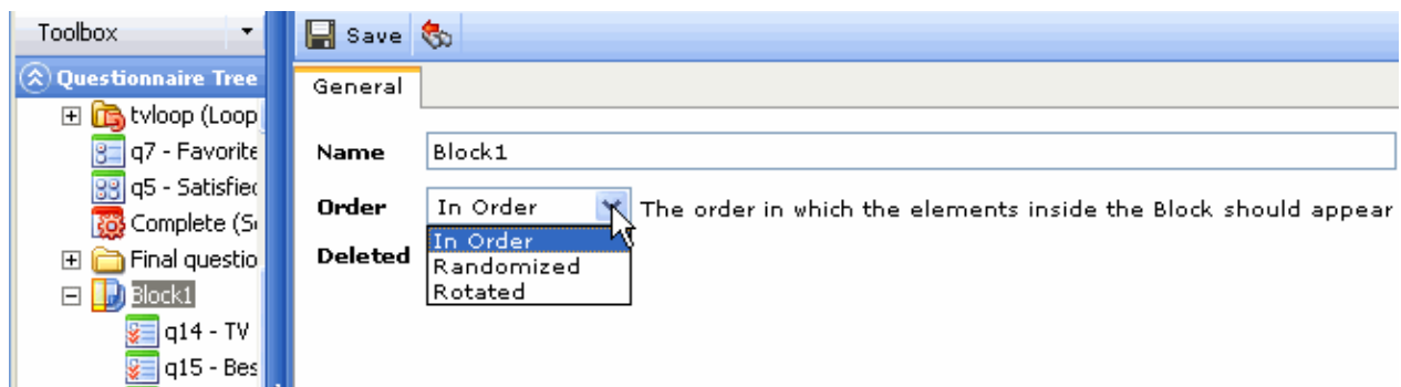
Figure 315 Setting up a Block object
