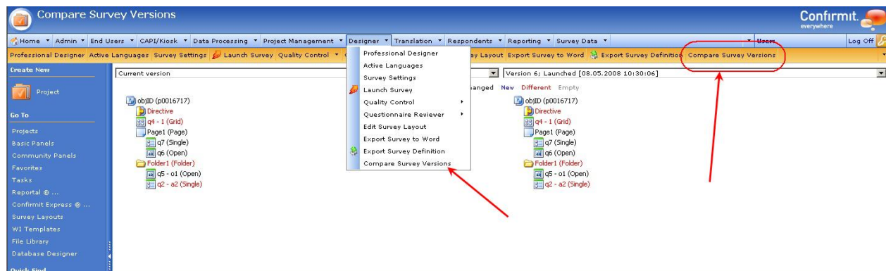
Figure 555 Example of the Survey Versions Comparison window
