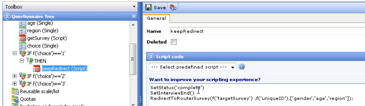
Figure 401 Example of a RedirectToRouterSurvey script
