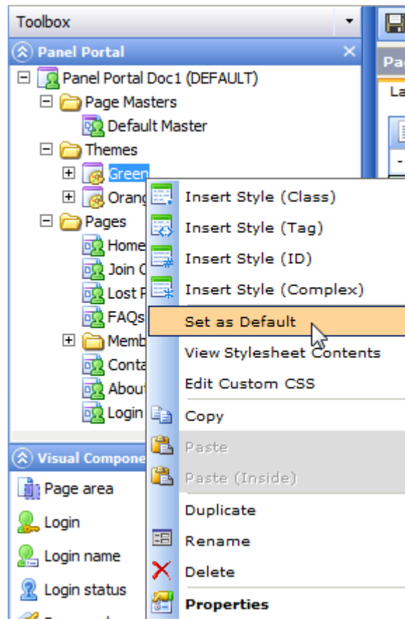
Figure 634 Setting a theme as Default
