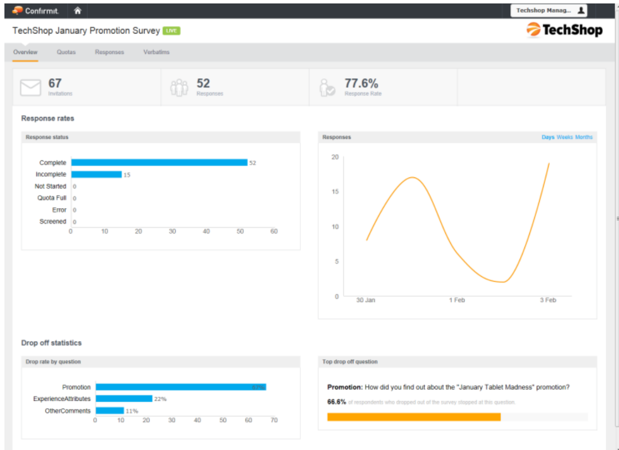
Figure 702 The Overview tab page layout
