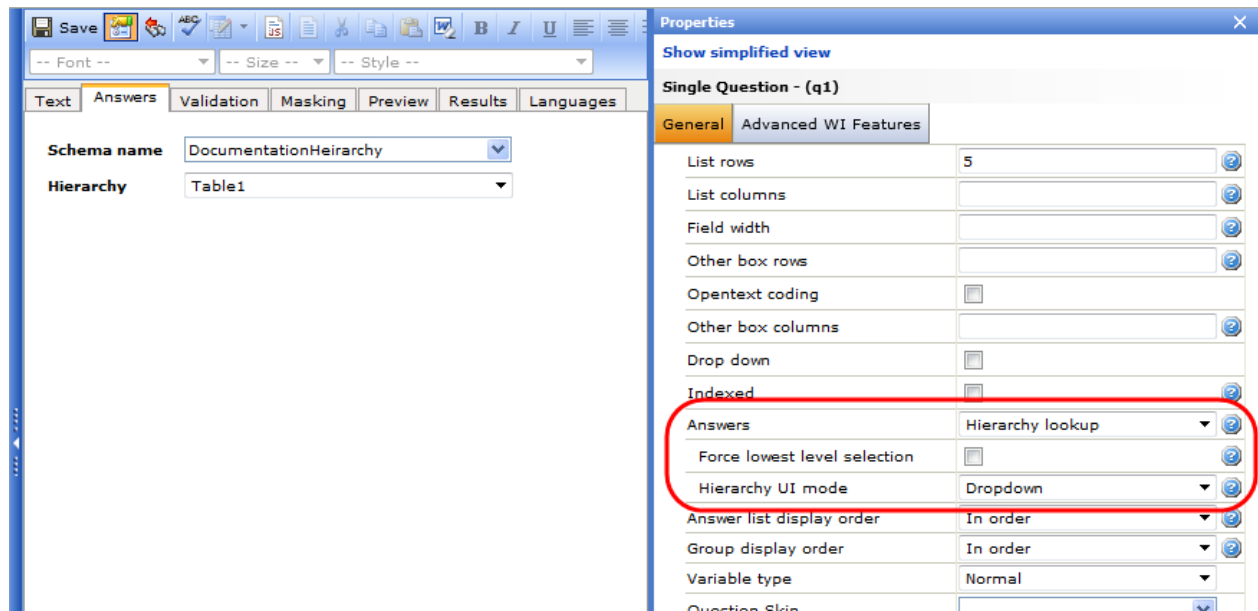
Figure 449 Selecting the Hierarchy for a "Hierarchy lookup" question type
