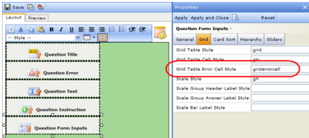
Figure 312 Specifying the Grid Table Error Cell Style
