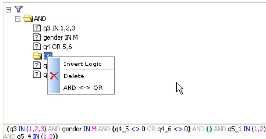
Figure 790 Inverting the logic or switching between AND and OR
