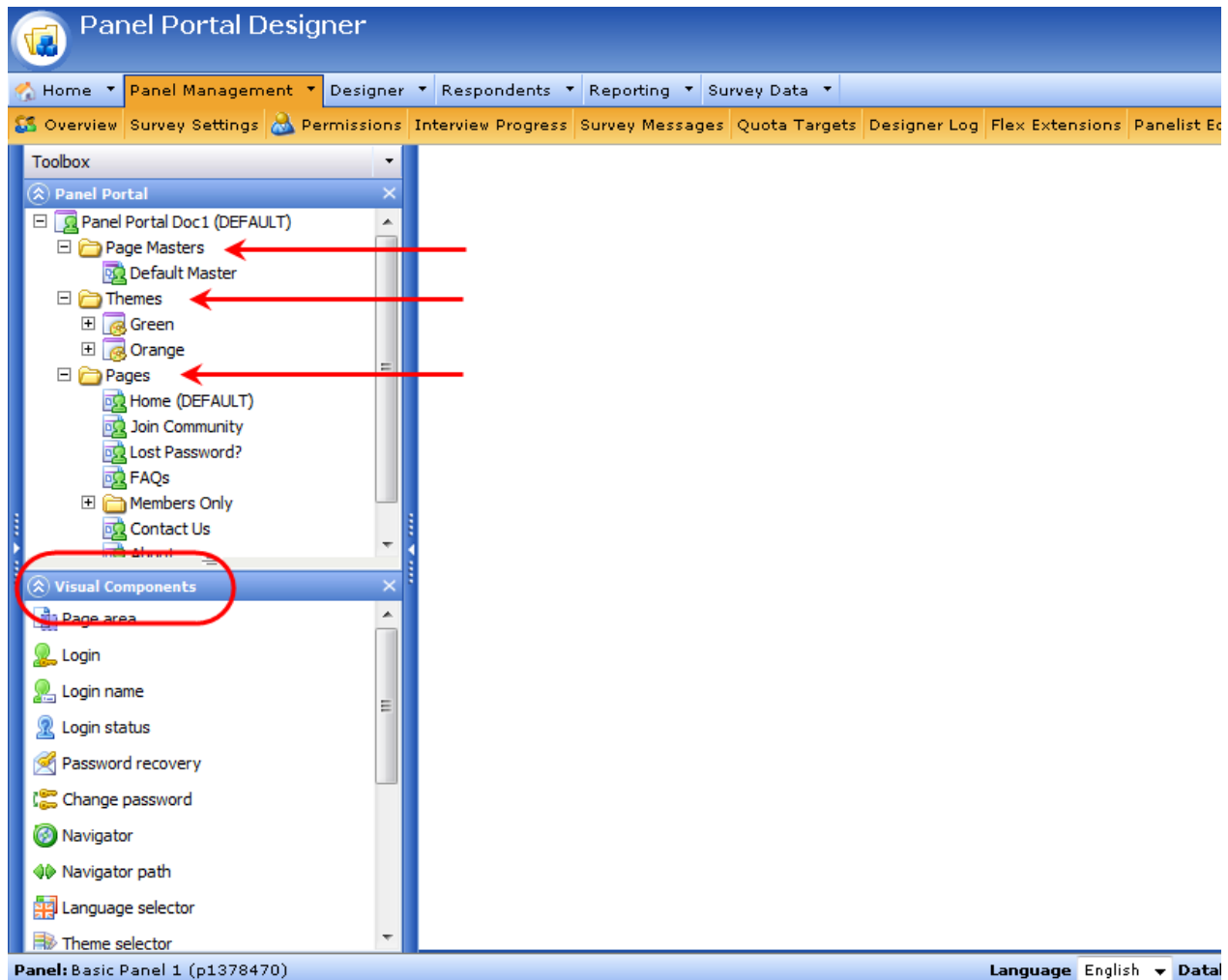
Figure 630 The toolboxes inside Portal Designer
