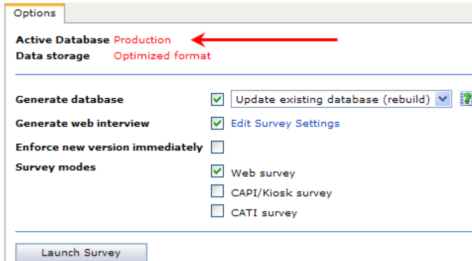
Figure 38 The active database shown in red text on the Launch Survey page
