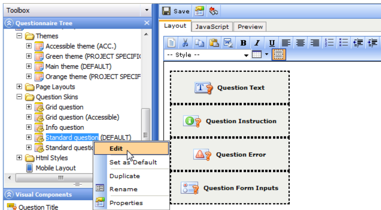
Figure 87 Editing a Question Skin
