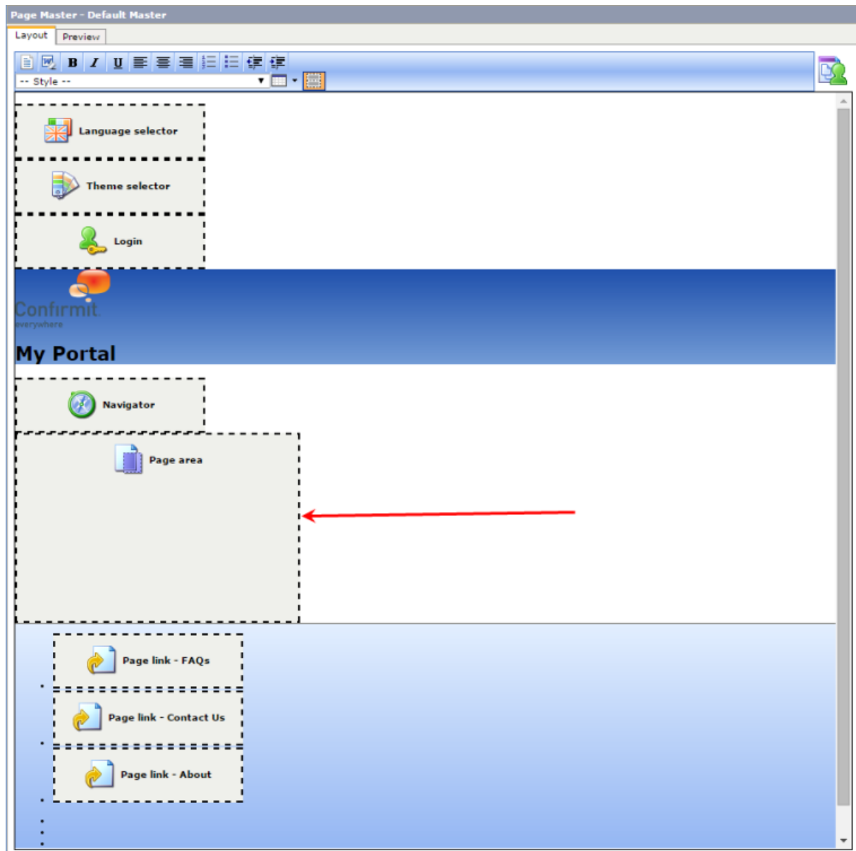
Figure 620 The location of the Page Area component in the page master
