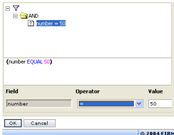
Figure 764 Defining a filter value for a numeric question
