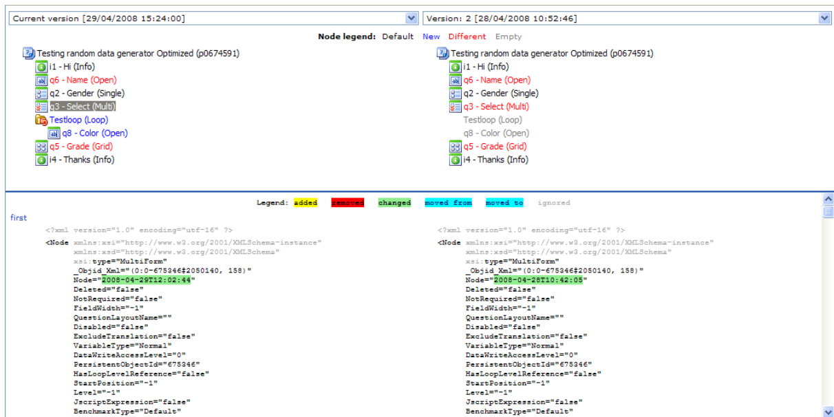
Figure 537 Example of the XML Comparison functionality
