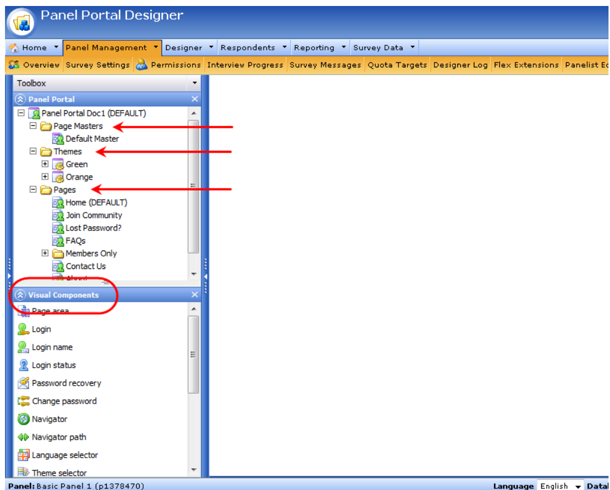
Figure 611 The toolboxes inside Portal Designer
