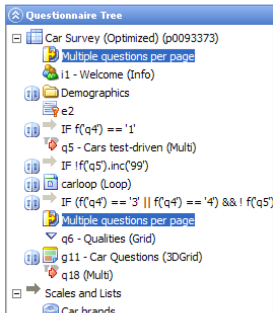
Figure 275 Example of a multiple questions directive
