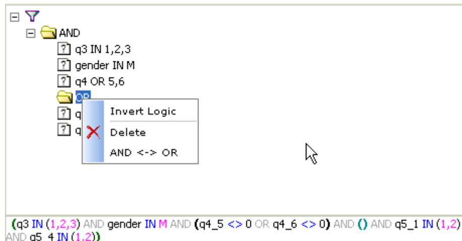
Figure 763 Inverting the logic or switching between AND and OR
