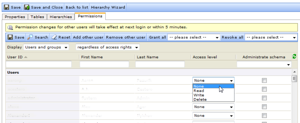
Figure 438 Example of the Access Rights tab for a table
