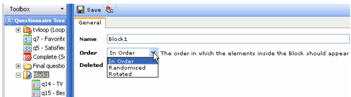
Figure 308 Setting up a Block object
