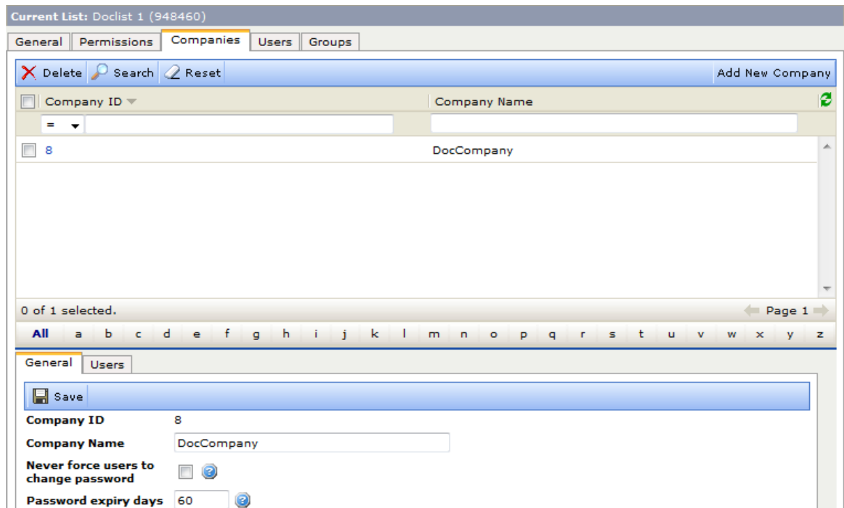
Figure 824 Example of the Companies tab
