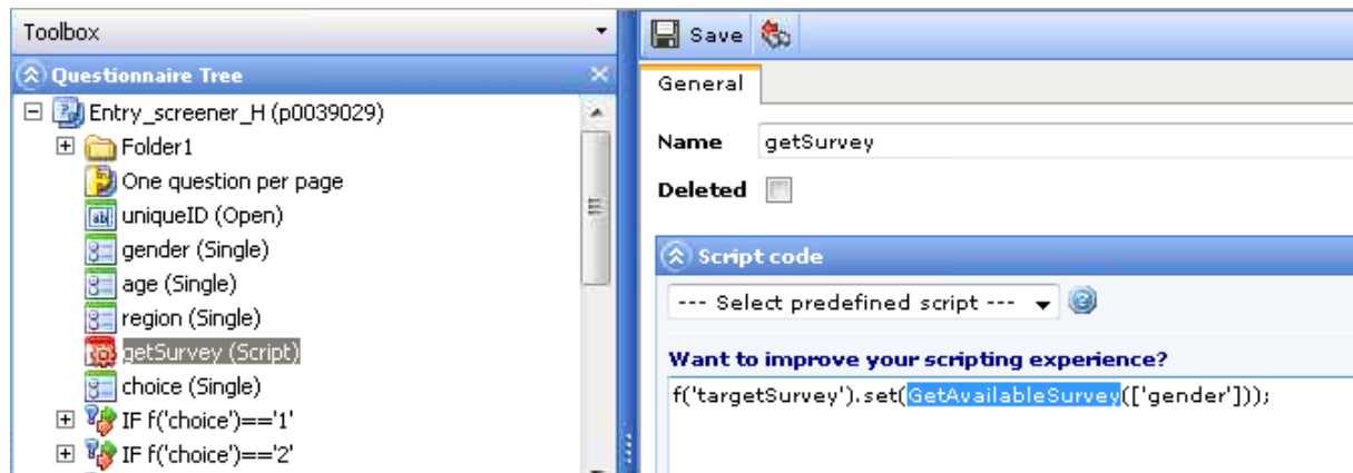
Figure 408 Example of the GetAvailableSurvey script in use
