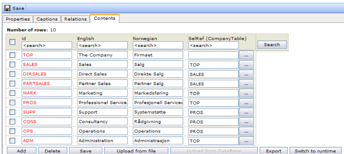
Figure 452 A self-referencing table
