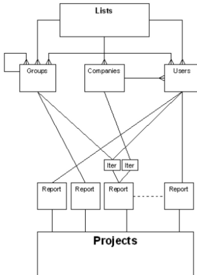
Figure 818 The End User administration interface layout
