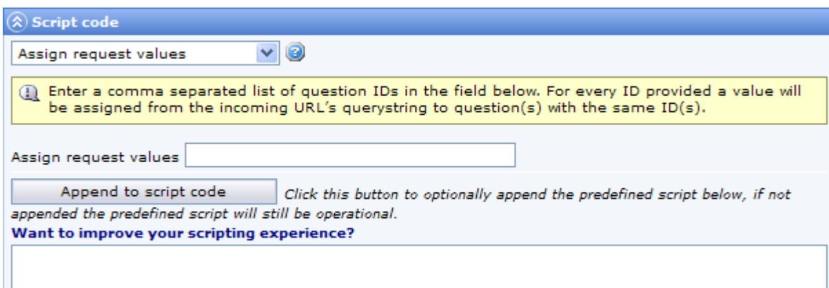
Figure 294 Using the Assign Request Values predefined script
