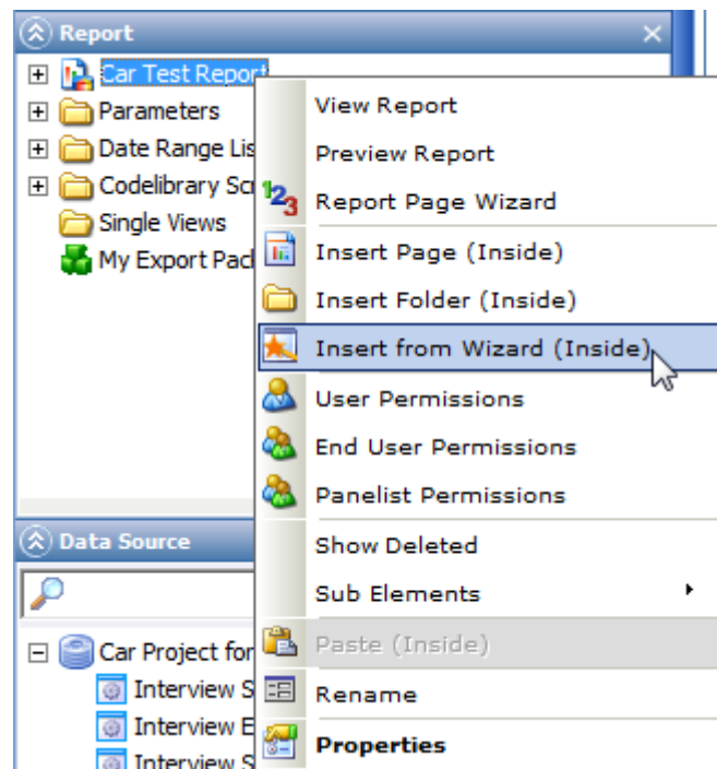
Figure 771 Inserting an object into an existing report using a Wizard Script
