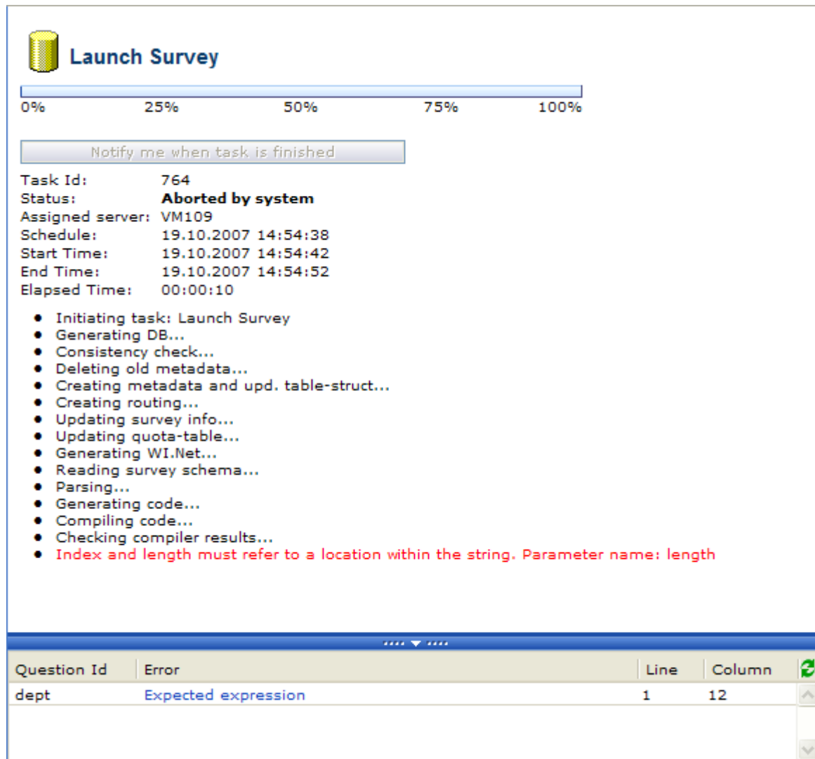
Figure 565 Example of a script error frame with an error link
