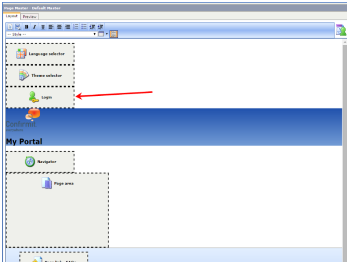
Figure 654 Example of a page master with the Login element
