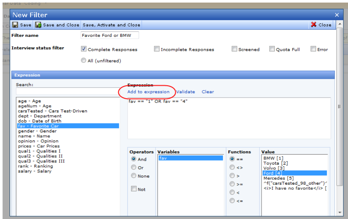
Figure 704 Creating the filter expression
