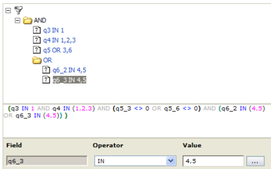
Figure 802 The final filter expression
