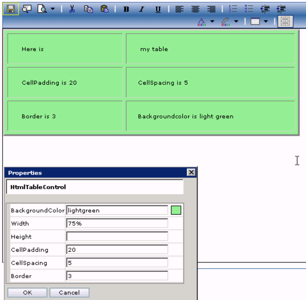
Figure 678 More table settings
