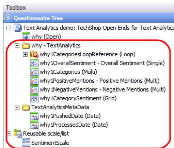
Figure 354 Example of the questionnaire set up for processing
