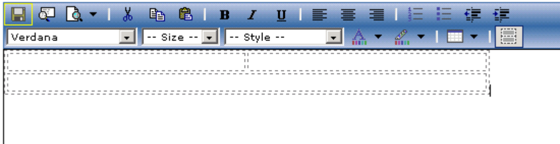
Figure 699 Merged cells
