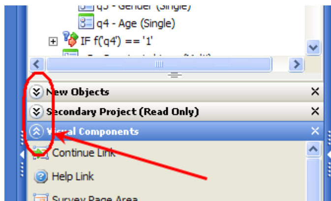
Figure 22 Collapse toolboxes
