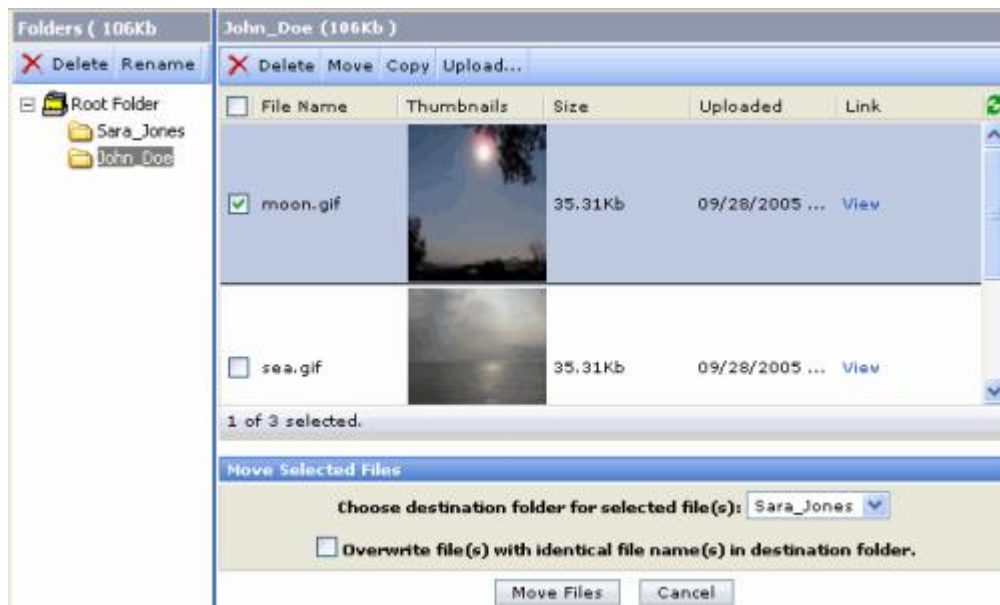
Figure 166 Moving files
