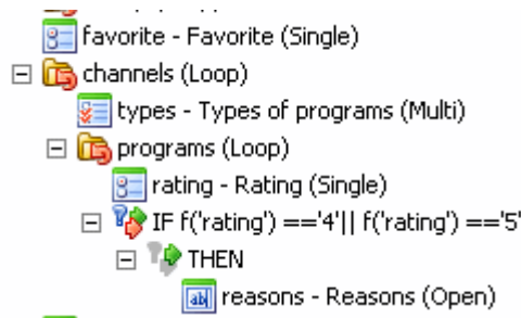
Figure 508 Nested loops
