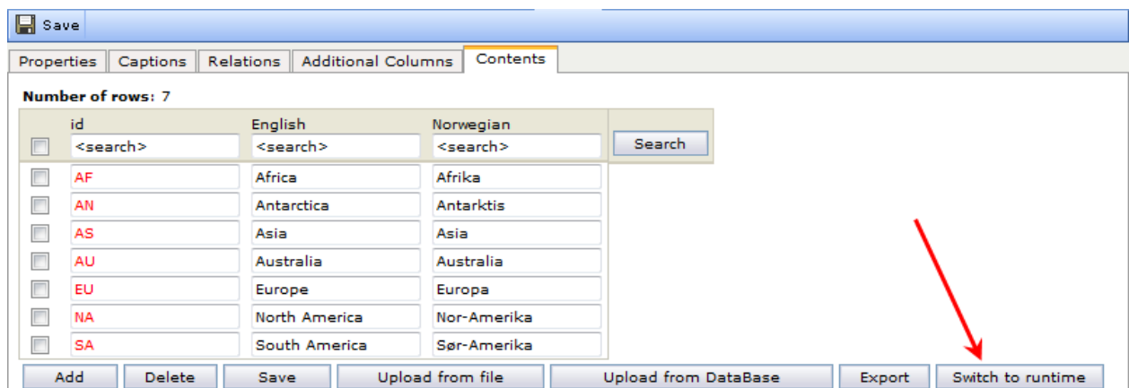
Figure 443 Runtime mode
