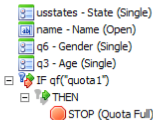
Figure 403 Quota Condition
