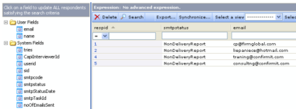
Figure 620 Respondent Editor
