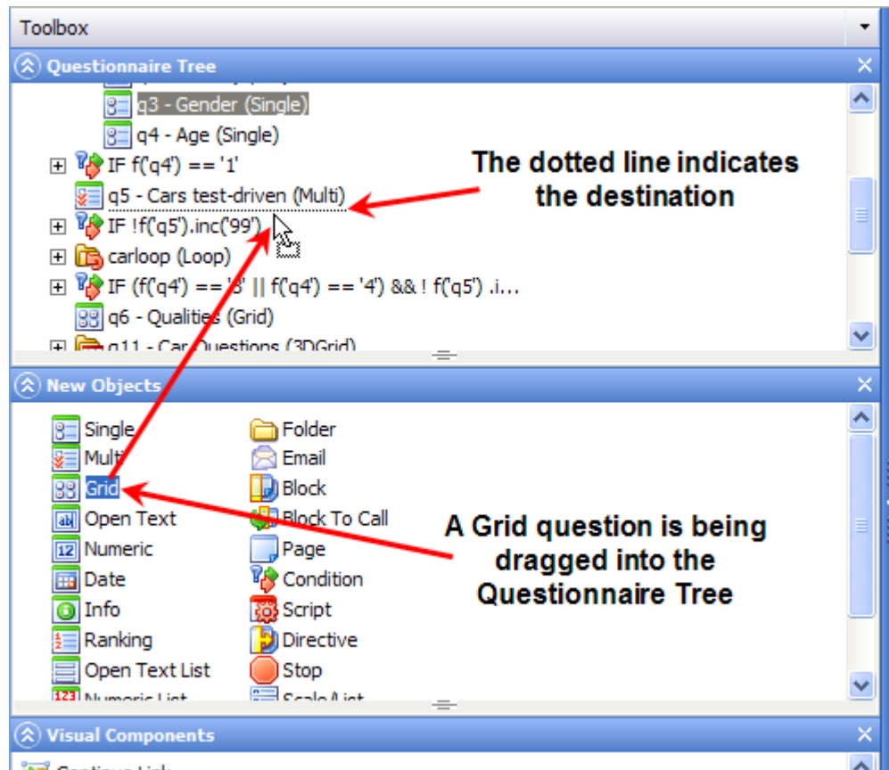
Figure 27 Drag-and-Drop operations
