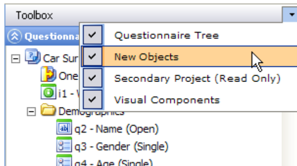
Figure 21 Removing toolboxes
