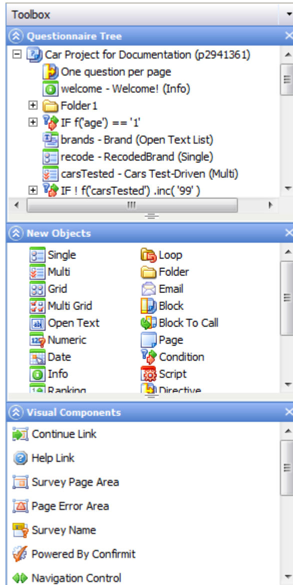
Figure 20 The Toolboxes
