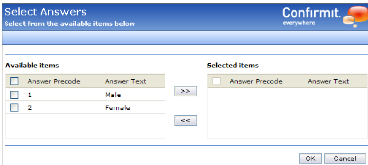
Figure 638 Excluding samples
