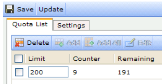
Figure 395 Global Quota
